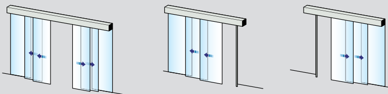
Wall mounted, doors and side screens
